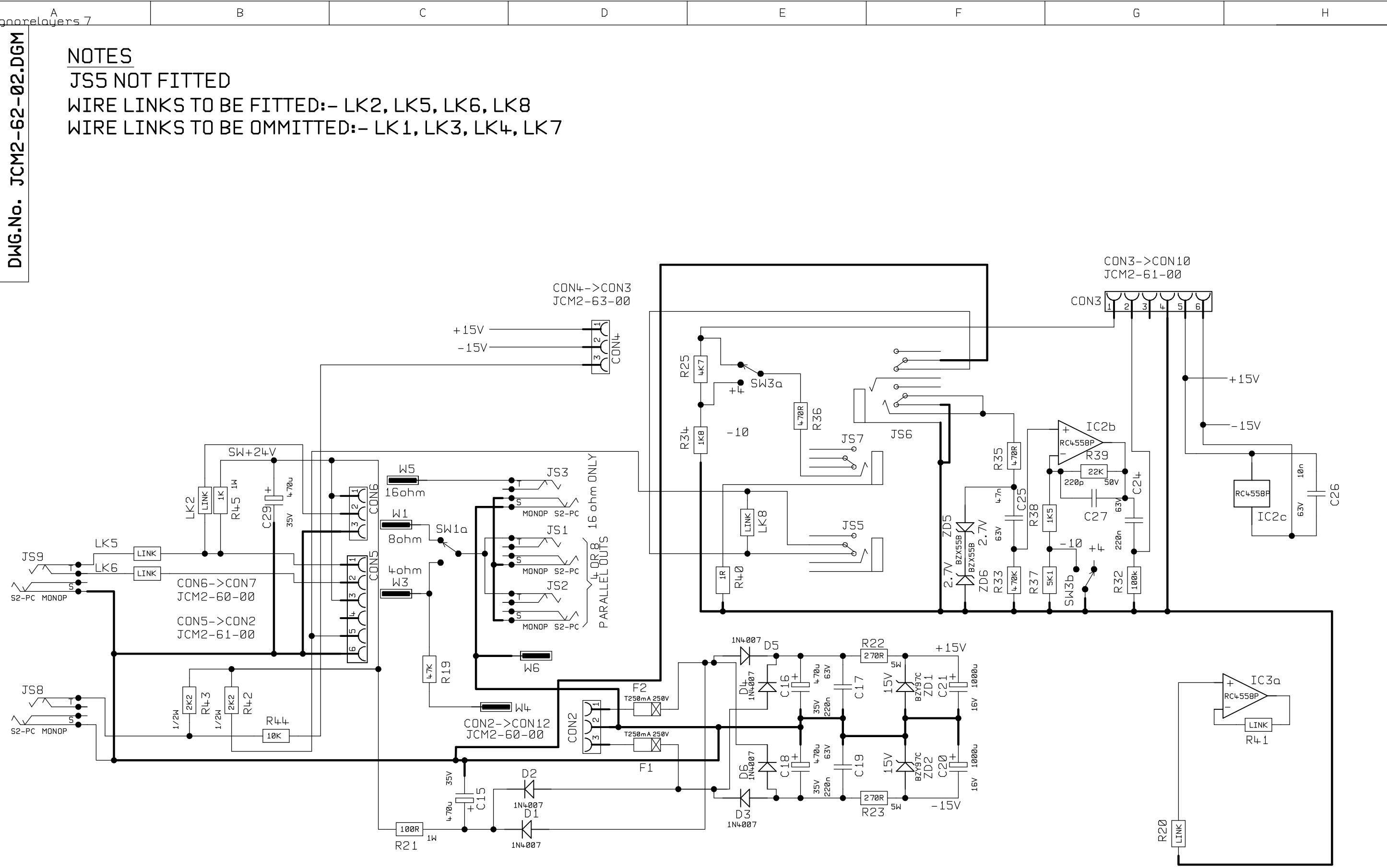
GENERIC PCB JCM2-62-00.ART SEE JCM2-69-00.DGM FOR DESIGN SCHEMATIC ALL OTHER DESIGNATIONS (EXCEPT REQUIRED LINKS) SHOULD BE UNFILLED
